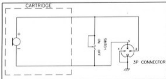
CIRCUIT
